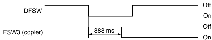
Timing chart 1-3-4
