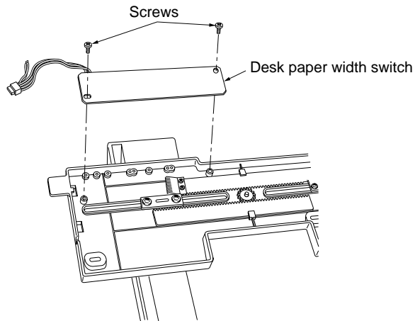
Figure 1-4-8 Detaching the desk paper width switch
