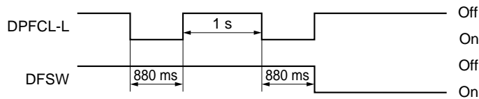
Timing chart 1-3-2
